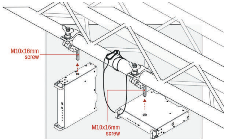
Truss Mounting (HDMI20-OPTC-RX220-Pro)
