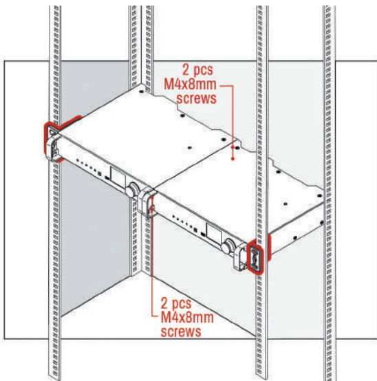
Mounting as a Standard Rack Installation (HDMI20-OPTC-TX220-Pro)
