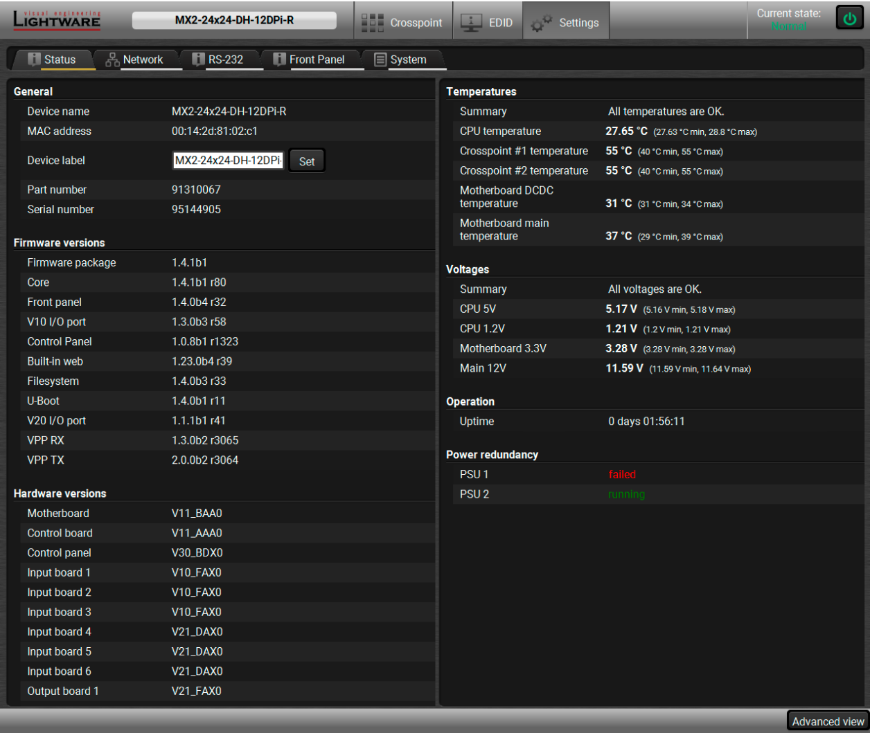
Status Tab in the Settings Menu
