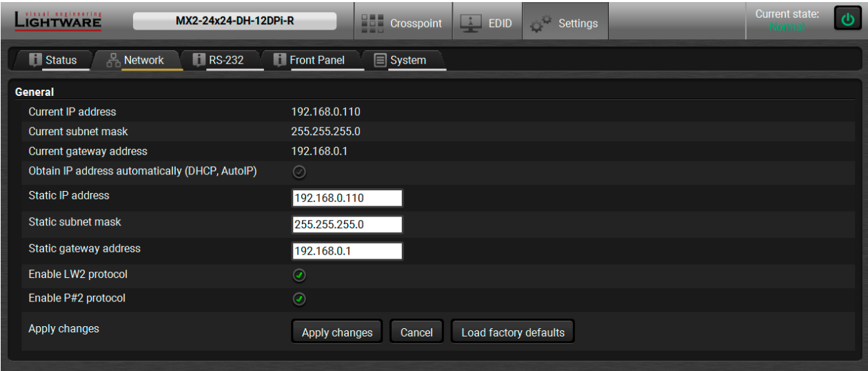
Network Tab in the Settings Menu
